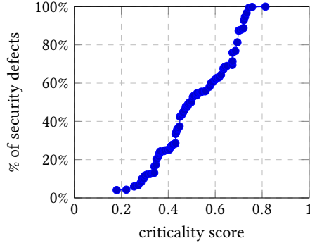
Figure 5: CDF of the severity of security defects
