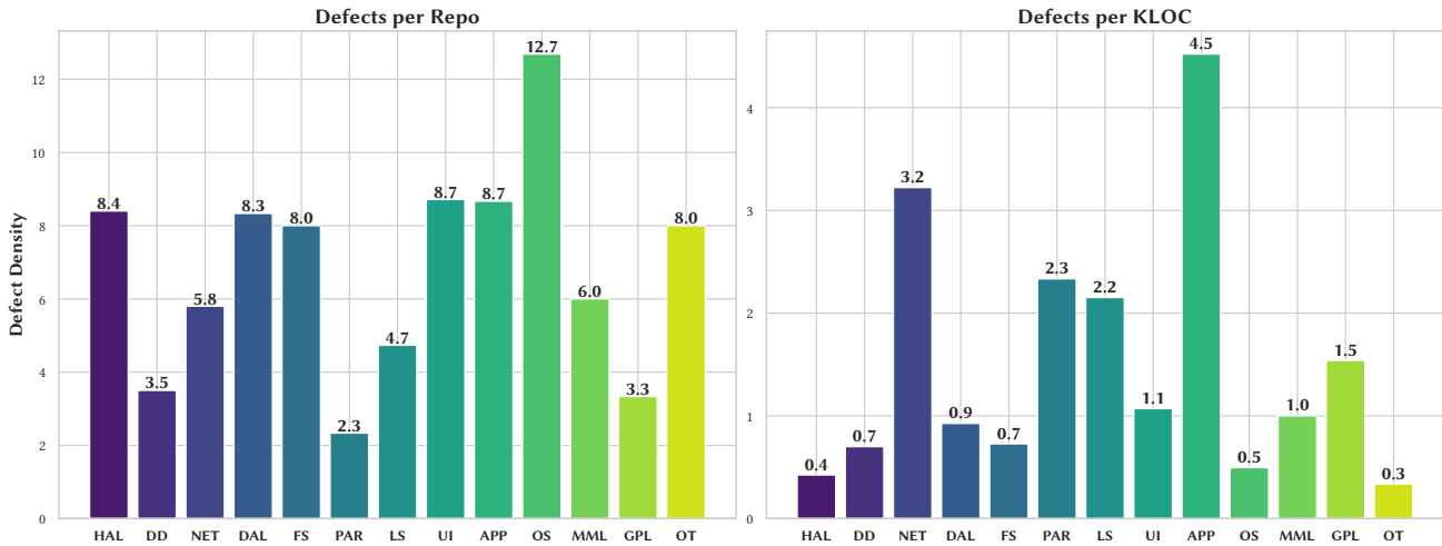
Figure 10: Defect density per number of repositories and KLOC across EMBOSS types
