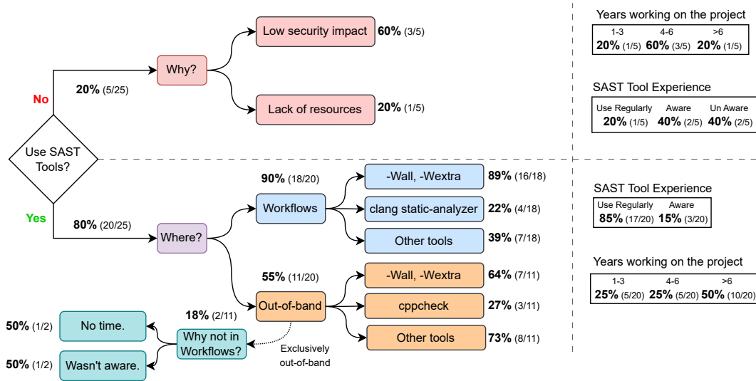
Figure 2: Summary of our developer survey on the use of SAST tools.
