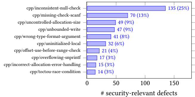
Figure 4: Top 10 CodeQL queries by # of security-relevant defects found. (Counts and Percentages)
