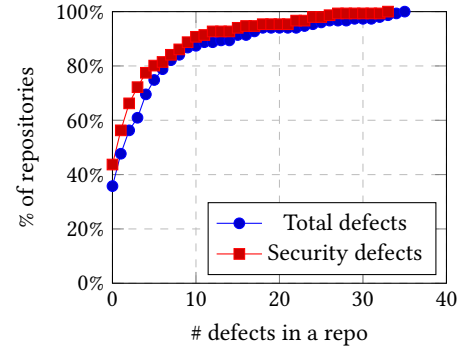
Figure 3: CDFs of # of all and security-relevant defects in a repository.
