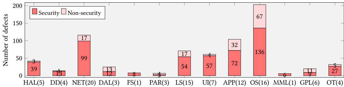
Figure 7: Number of defects of each type in EMOSS of various categories (Table 1). The number next to the category indicates the number of repositories containing at least one defect.
