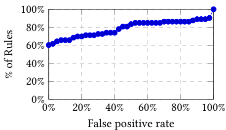
Figure 8: CDF of the false positive rates of rules
