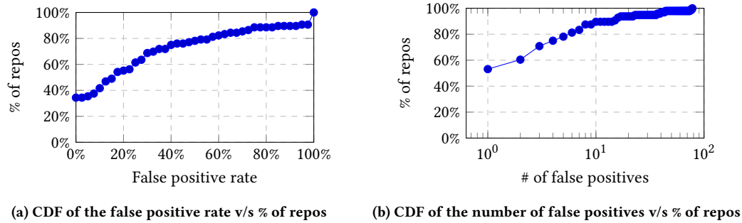
Figure 9: CDFs of the rate and number of false positives v/s percentage of repositories (repos).
